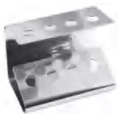
MR083 Weight:230g Thickness: 1.2 Size:L110*W67*H88mm
